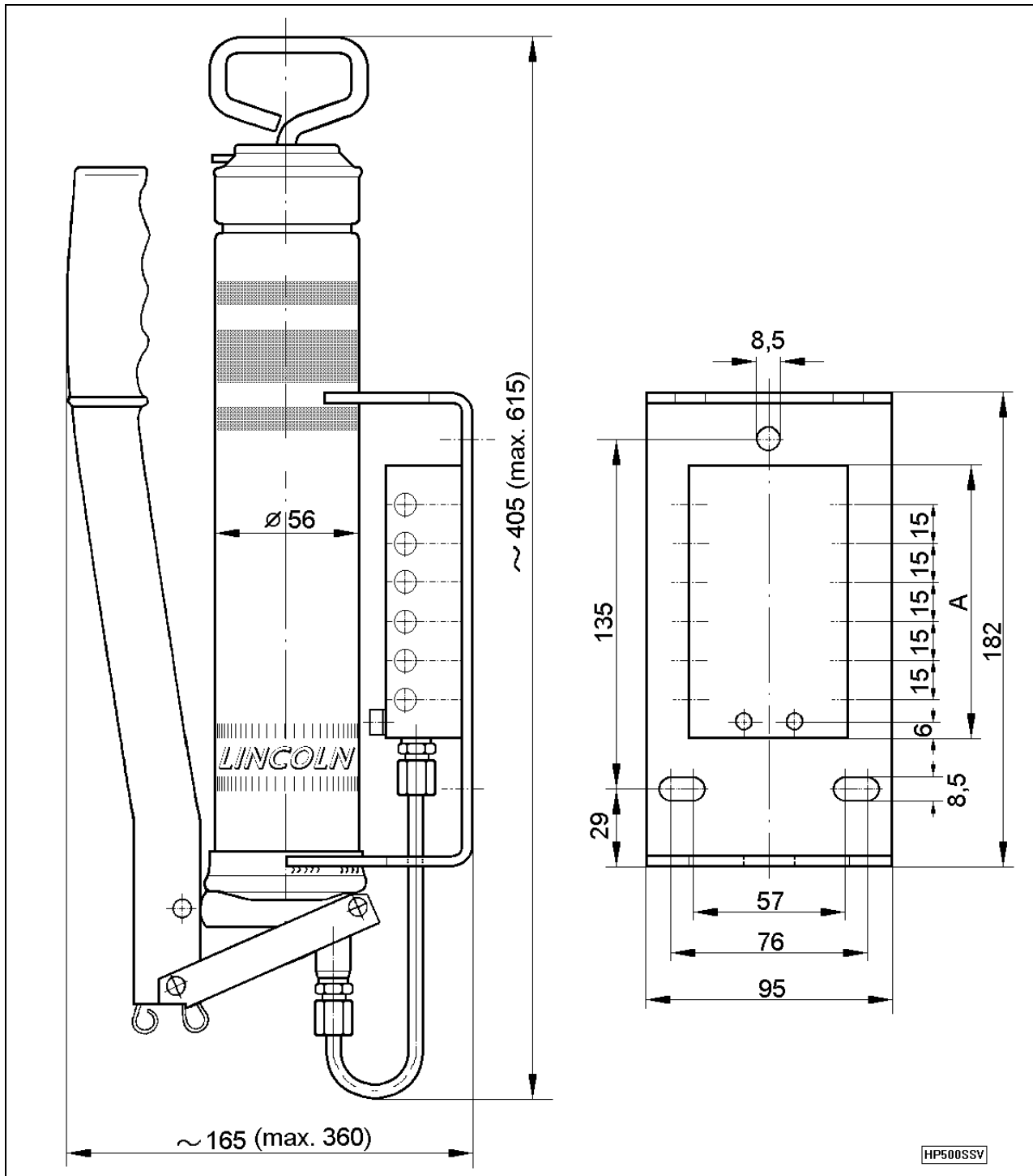
Stationary manual grease pump with integrated progressive metering device
